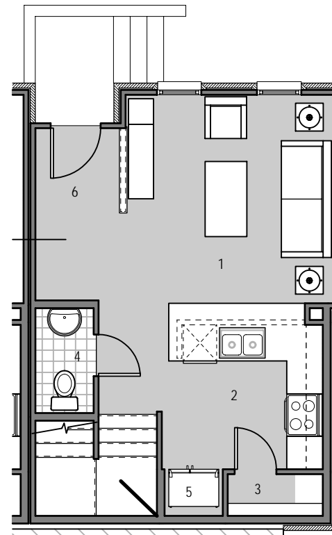
01 FLOOR PLAN - UNIT C1 / LEVEL 1 C1 SCALE: 1/8" = 1'-0"
