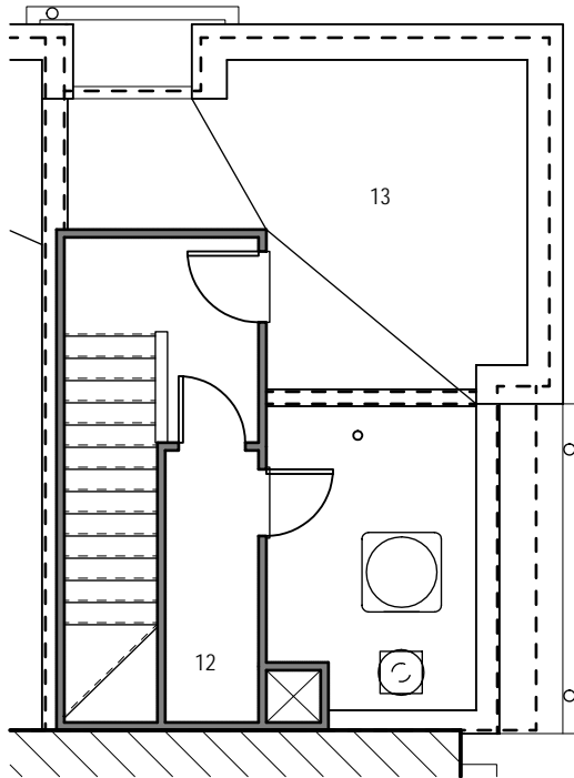
03 FLOOR PLAN - UNIT C1 / TERRACE C1 SCALE: 1/8" = 1'-0"
